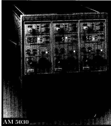
Three AM 5030s in a TM 5003 mainframe. Six AM 5030s will plug into a TM 5006A. All current measurement parameters can be set using a GPIB controller.
