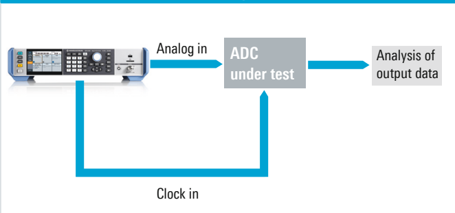
Compact ADC test setup with a single R&S®SMA100B with an integrated second source.
