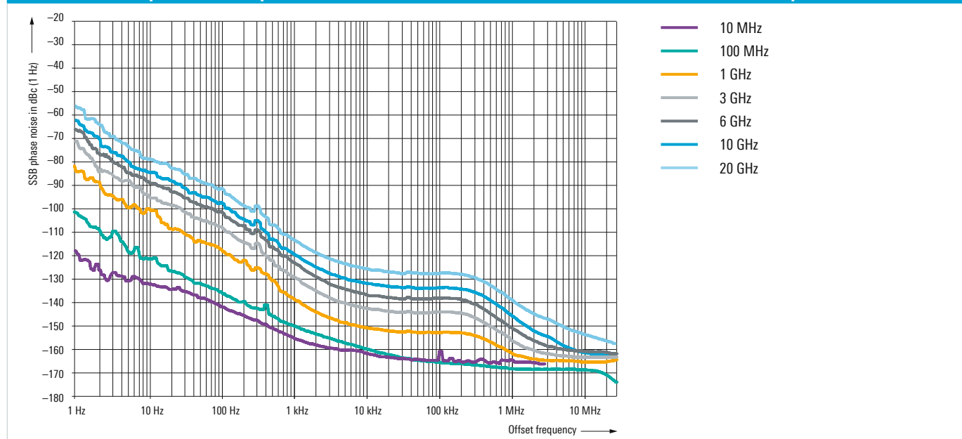
Measured SSB phase noise performance of the R&S®SMA100B with R&S®SMAB-B711 option
