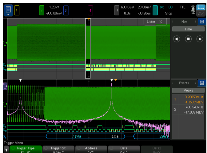
Figure 37b. Gated FFT time correlating the FSK frequency hopping with an I 2 C command (write 7 @ 0x71 data 10).
