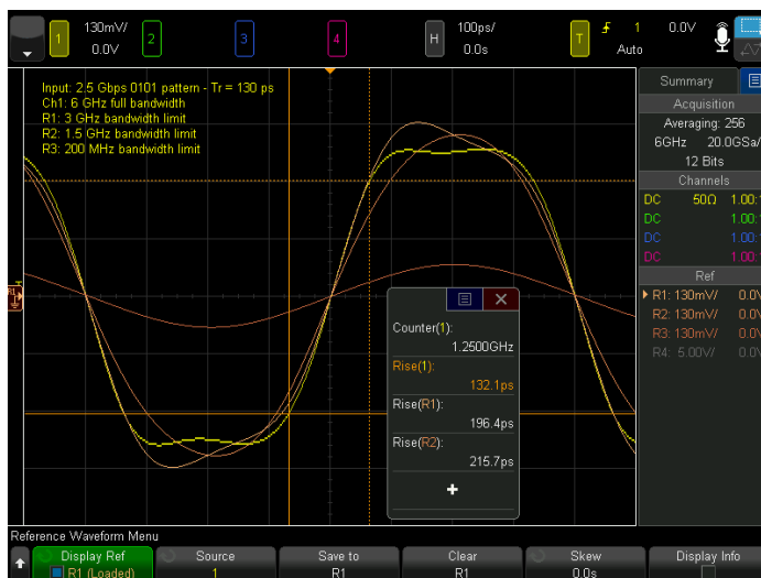
Figure 51. Reference waveforms.
