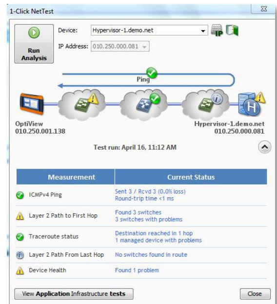
1-Click NetTest
