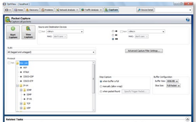
Packet Capture
