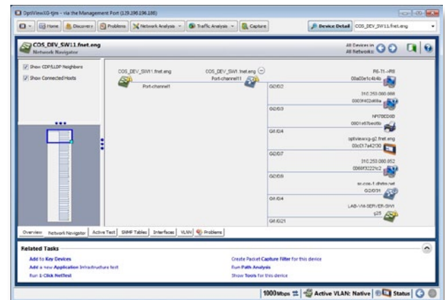
Network Navigator
