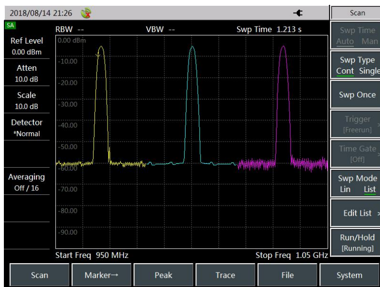
Figure 5-4 List sweep display
