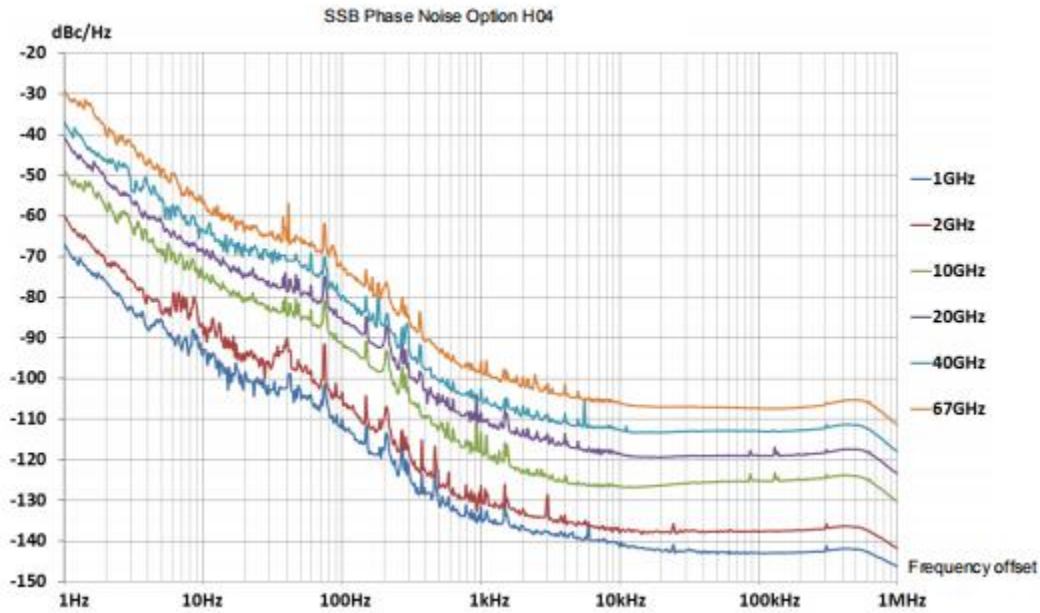
Fig. 3.1 SSB Phase Noise
