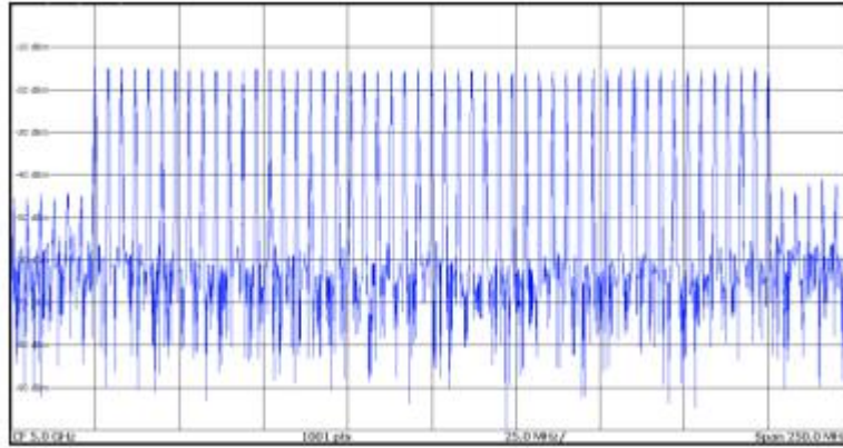
Fig. 3.3 5GHz Carrier 200MHz Modulation Bandwidth Multi-tone Signal
