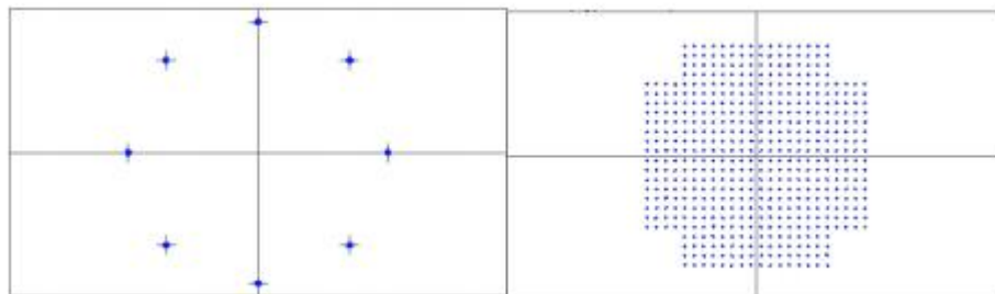
Fig.3.7 8PSK and 512QAM
