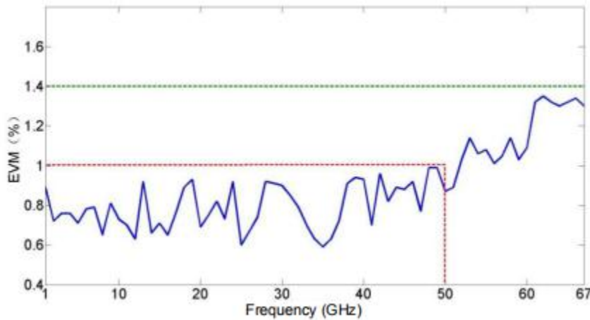
Fig.3.6 Vector Modulation Accuracy
