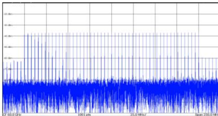
Fig. 3.4 60GHz Carrier 200MHz Modulation Bandwidth Multi-tone Signal
